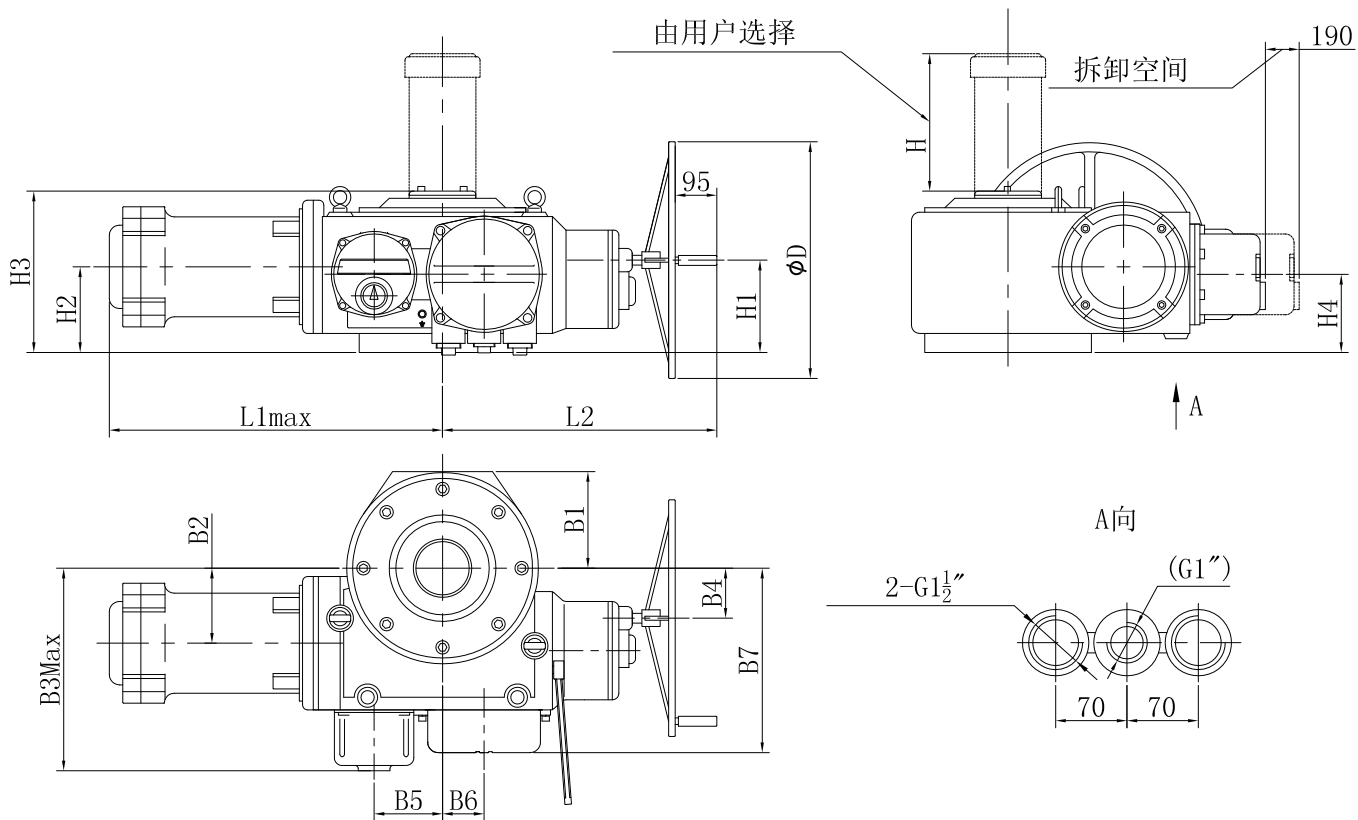
SMC-3~4基本型外形尺寸
